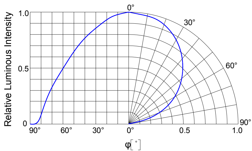
Fig.2 Radiation Characteristic
