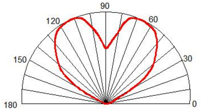
Fig.8 Radiation pattern@350mA
