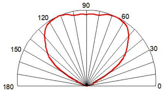
Fig.8 Radiation pattern@30mA
