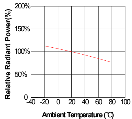
Fig.4 Relative Radiant Power VS Ambient Temperature
