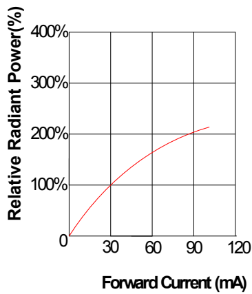
Fig.1 Relative Radiant Power VS Forward Current(Ta=25°C) Fig.2 Forward Current VS Forward Voltage (Ta=25°C)
