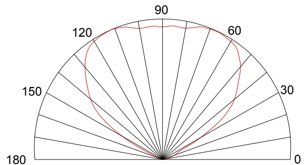
Fig.8 Radiation pattern@30mA
