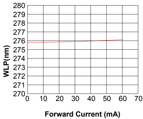
Fig.5 Peak Wavelength VS Forward Current
