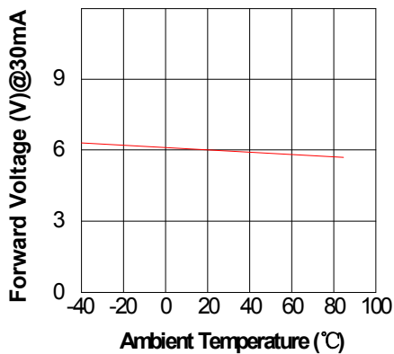
Fig.3 Forward Voltage VS Ambient Temperature
