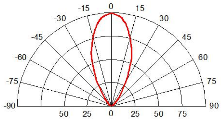
Fig.8 Radiation pattern@350mA
