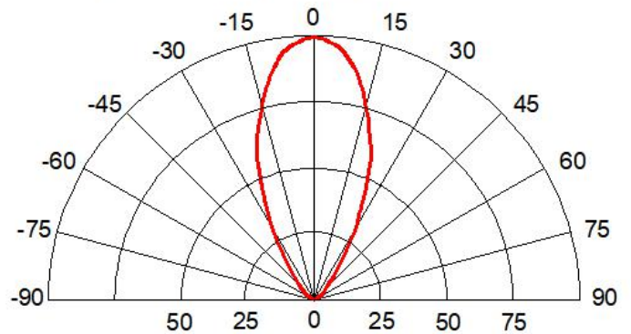
Fig.8 Radiation pattern@60mA
