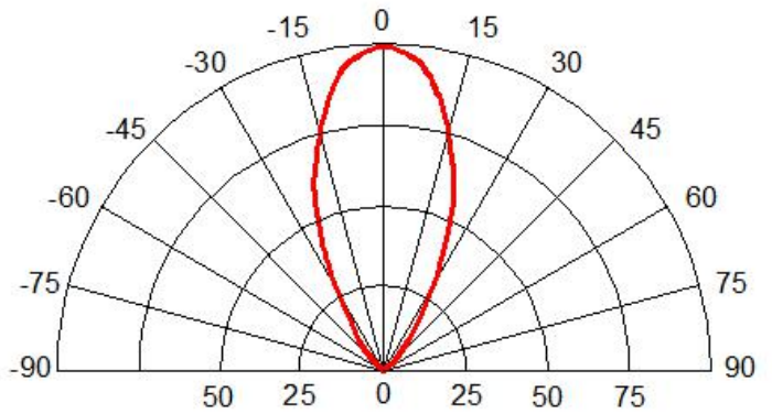
Fig.8 Radiation pattern@30mA
