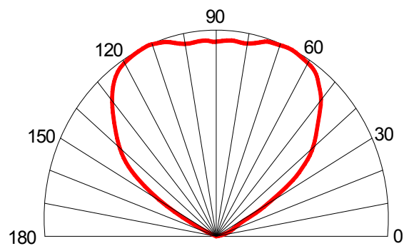
Fig.8 Radiation pattern@100mA
