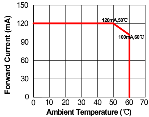
Fig.6 Forward Current VS Ambient Temperature
