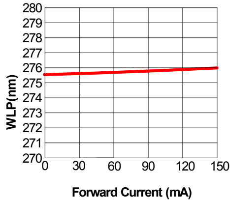
Fig.5 Peak Wavelength VS Forward Current
