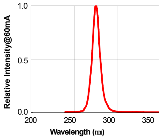
Fig.7 Relative Intensity VS WLP
