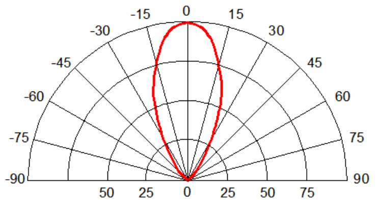
Fig.8 Radiation pattern@150mA
