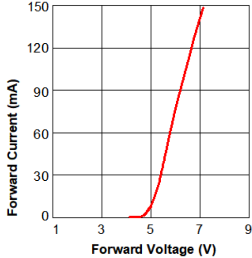
Fig.2 Forward Current VS Forward Voltage (Ta=25℃)
