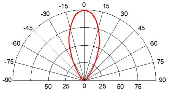
Fig.8 Radiation pattern@60mA
