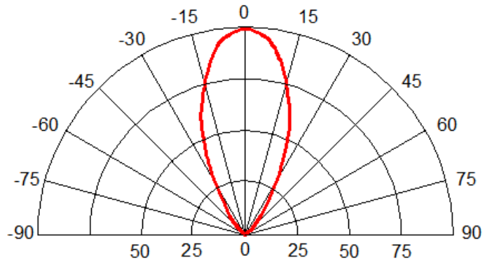
Fig.8 Radiation pattern@30mA
