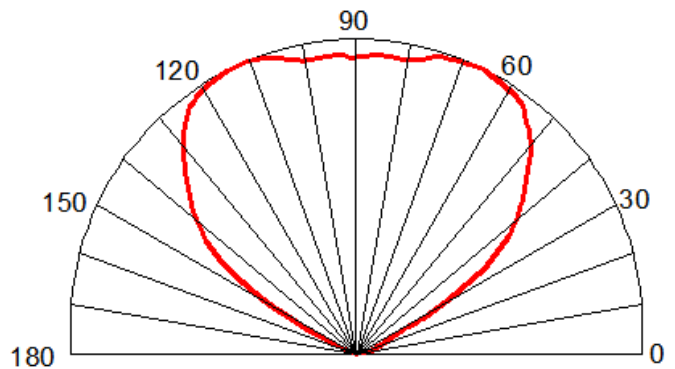
Fig.8 Radiation pattern@350mA
