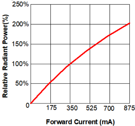
Fig.1 Relative Radiant Power VS Forward Current
