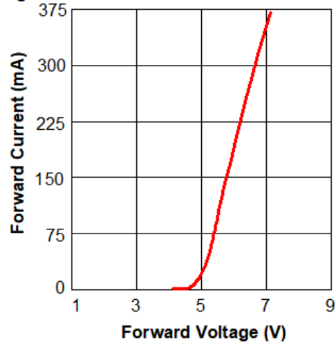
Fig.2 Forward Current VS Forward Voltage (Ta=25°C)
