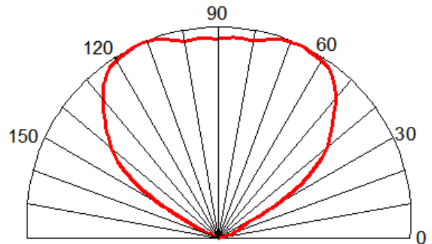
Fig.8 Radiation pattern@150mA
