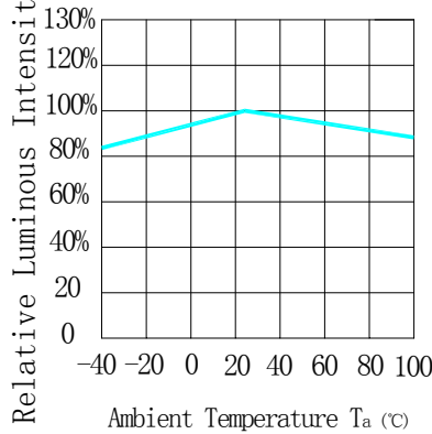
Fig.4 Relative Intensity Vs Ambient Temperature
