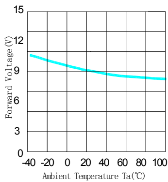
Fig.3 Forward Voltage Vs Ambient Temperature
