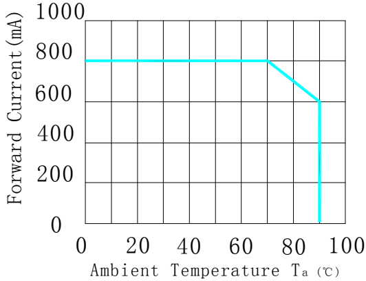
Fig.3 Forward Current Vs Ambient Temperature
