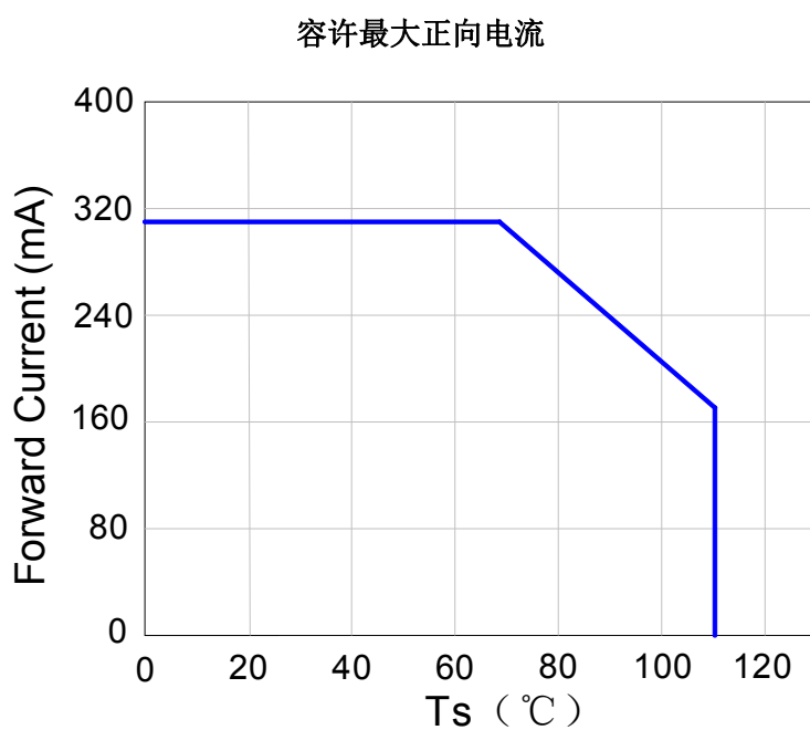
Fig.6 Max. Permissible Forward Current
