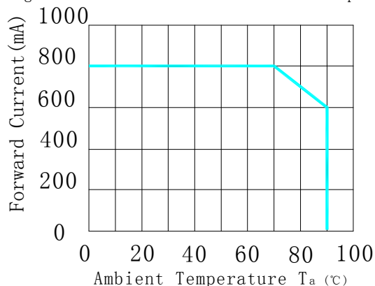
Fig.3 Forward Current Vs Ambient Temperature
