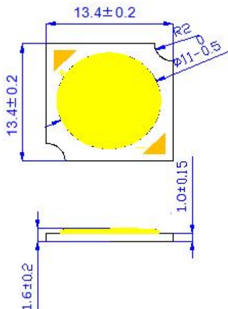
Outline dimensions
