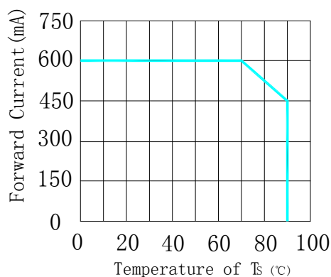
Fig.3 Forward Current Vs Temperature of T_s
