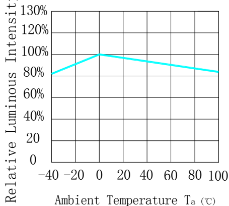
Fig.4 Relative Intensity Vs Ambient Temperature
