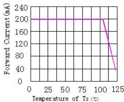
Fig.3 Max Driving Forward Current Vs Temperature of Ts
