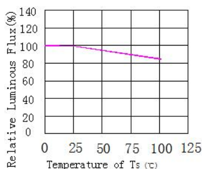
Fig.4 Relative Luminous Flux Vs Temperature of Ts (VF=24V)
