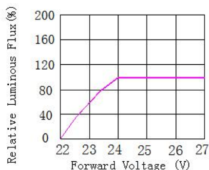
Fig. 2 Forward Voltage Vs Relative Luminous Flux
