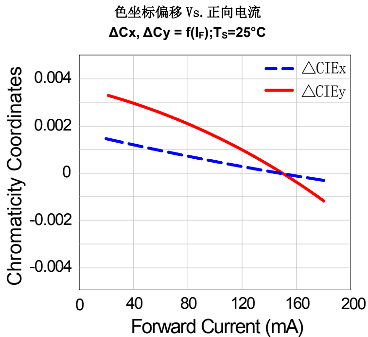
Fig.5 Chromaticity Coordinates Shift vs. Forward Current
