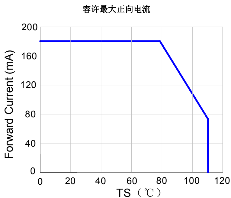
Fig.6 Max. Permissible Forward Current
